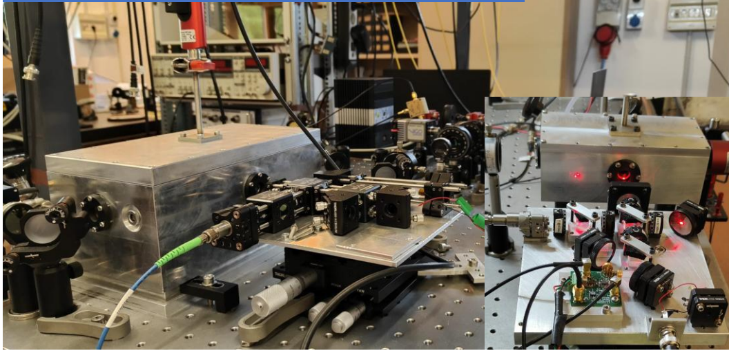
Photoacoustic Sensor
